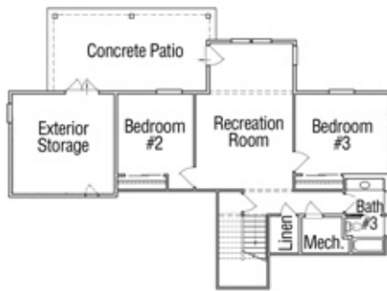
LOWER LEVEL
